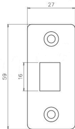
FACE PLATE
